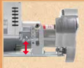
Hinged Plate
